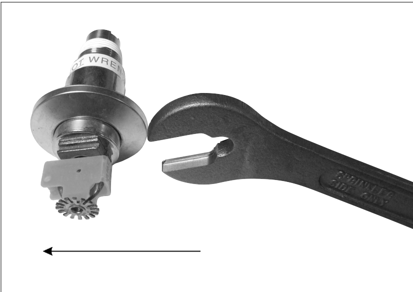
Fig. 10 - Model F3 or Model F3R Wrench
